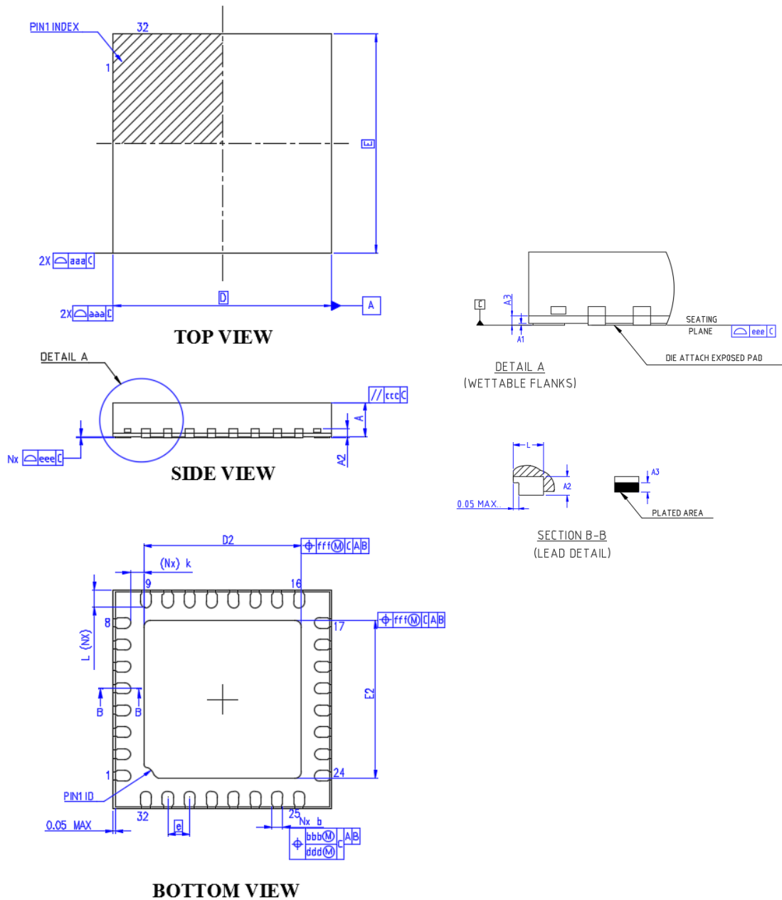
Figure 26. VFQFPN (5x5x1.00 mm) package outline
