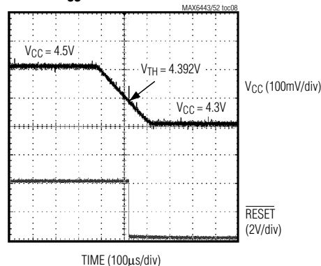
V_{CC} TO \overline{\text{RESET}} DELAY
