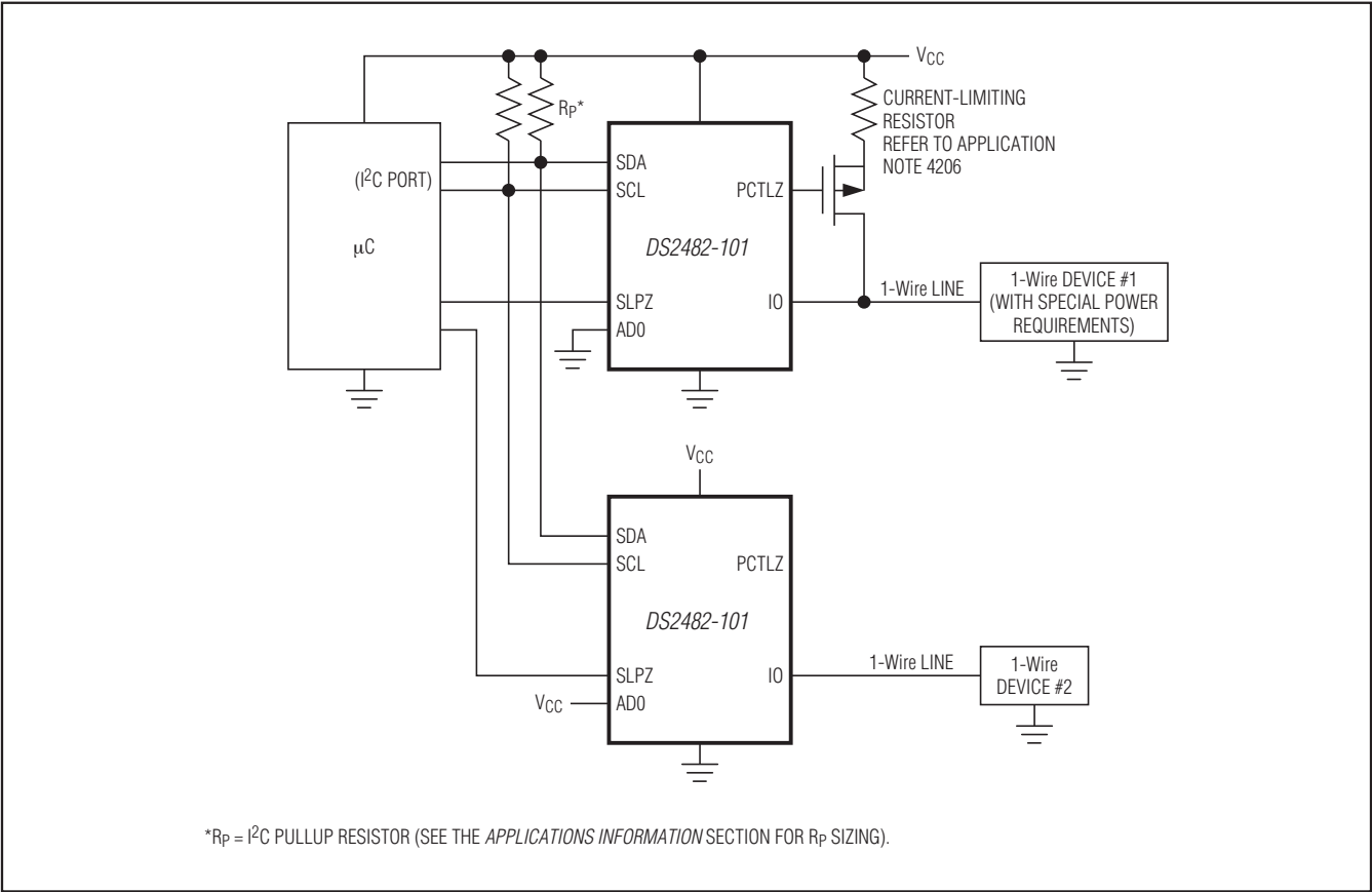
Figure 10. Application Schematic
