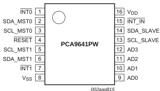
Fig 2. Pin configuration for TSSOP16
