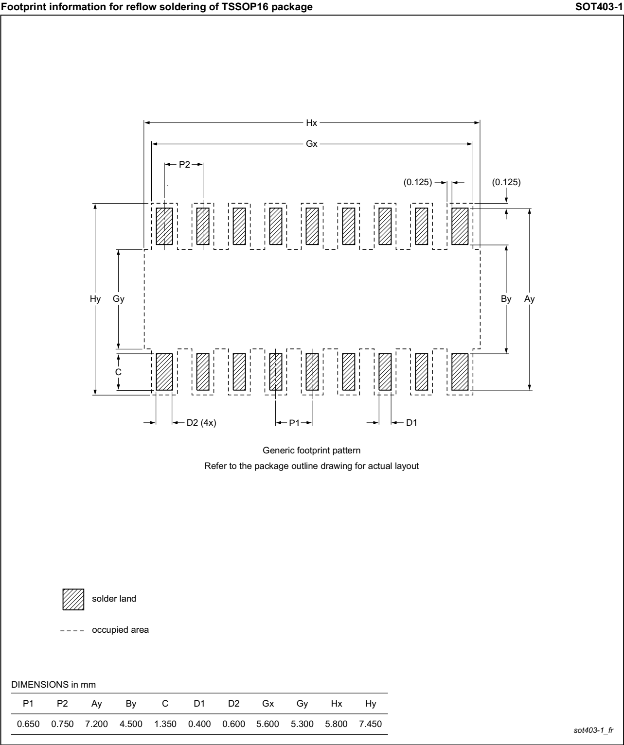
Fig 38. PCB footprint for SOT403-1 (TSSOP16); reflow soldering
