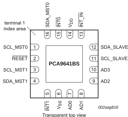
Fig 3. Pin configuration for HVQFN16
