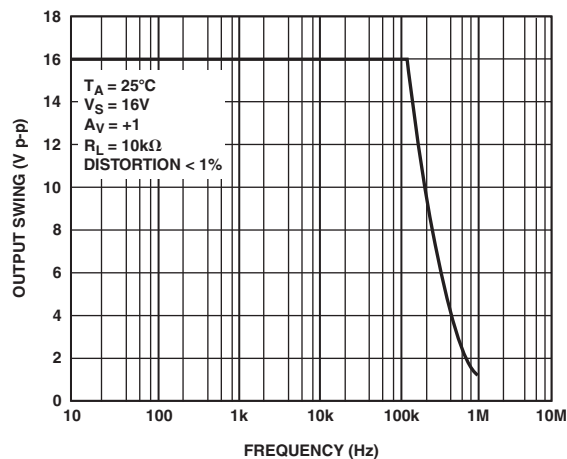
TPC 16. Closed-Loop Output Swing vs. Frequency
