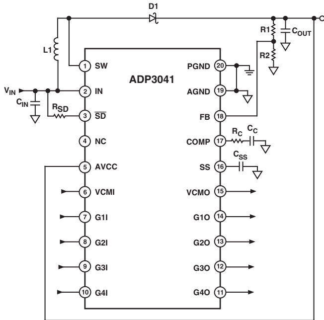
Figure 1. Typical Application
