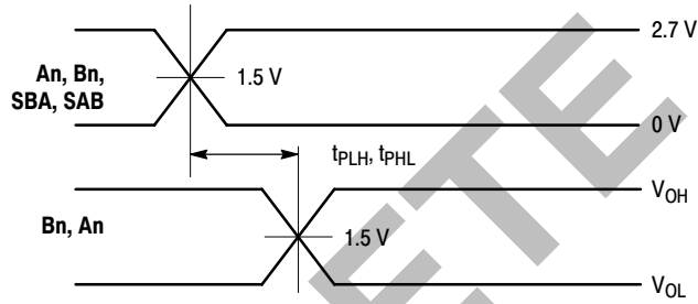
WAVEFORM 1 – SAB to B and SBA to A, An to Bn PROPAGATION DELAYS
