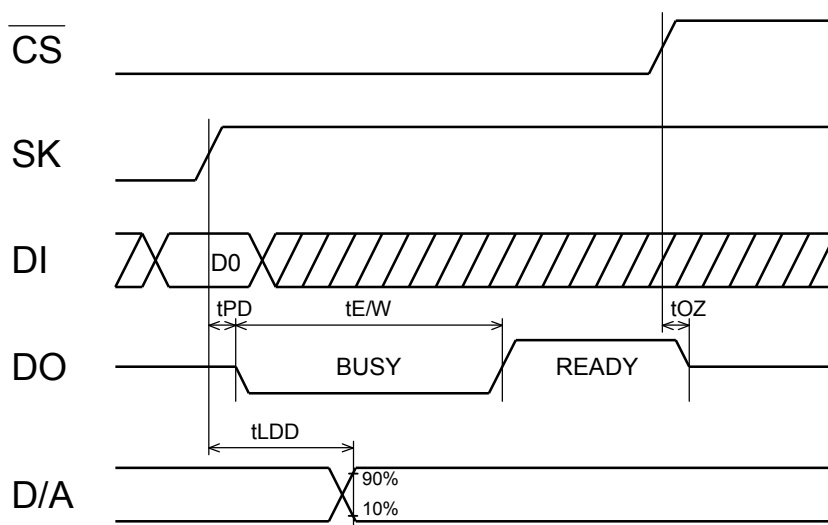
READY/ \overline{\text{BUSY}} signal output timing
