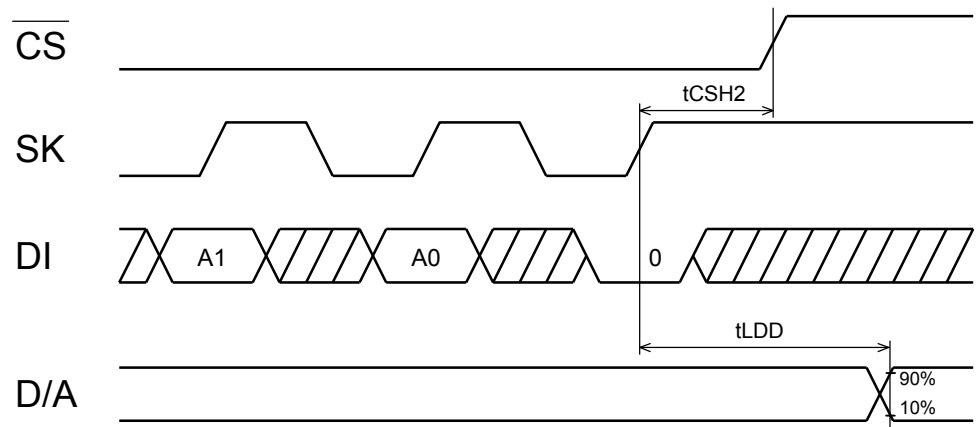
D/A converter output timing in CALL instruction
