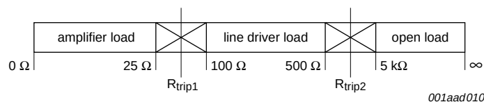
Fig 7. DC load detection limits (R PROG = 1500 Ω/1 %)
