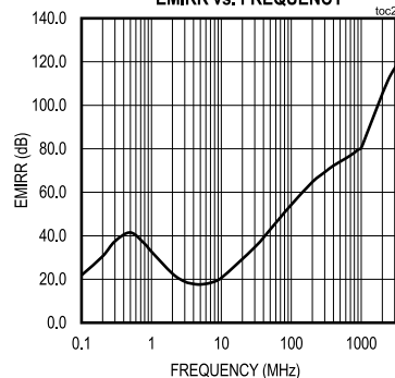
EMIRR vs. FREQUENCY
