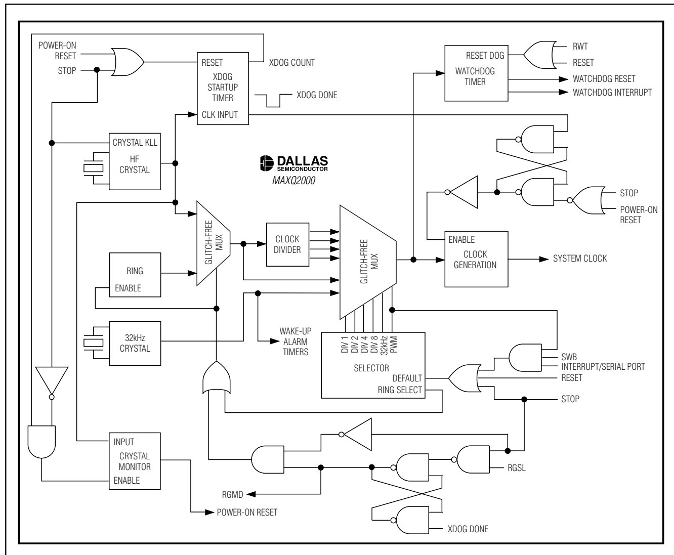
Figure 2. Clock Sources
