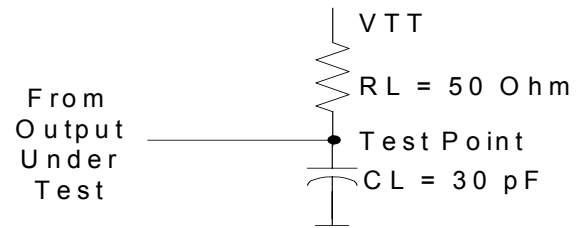
Figure 5. Load Circuit [8]
