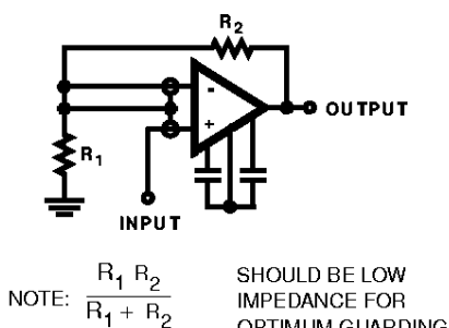
FIGURE 1C. NON-INVERTING AMPLIFIER
