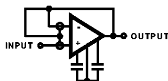
FIGURE 1B. FOLLOWER
