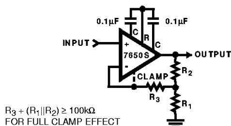
FIGURE 2. NON INVERTING AMPLIFIER WITH OPTIONAL CLAMP
