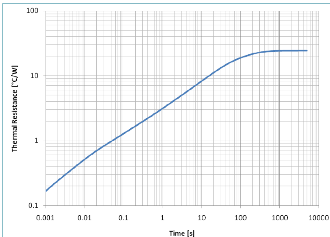
Figure 18. Transient thermal resistance R_{\theta JA} MC33932EK on 2s2p test board
