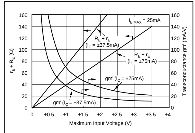
FIGURE 4. R_E + r_E Selection Curve.
