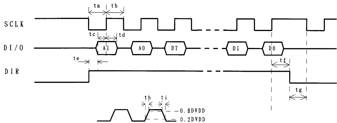
SCLK/DIR input
