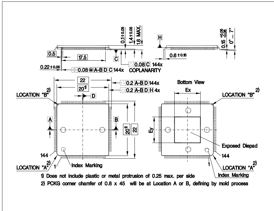
Figure 30 PG-LQFP-144-16I-23 (Plastic Green Thin Quad Flat Package)
