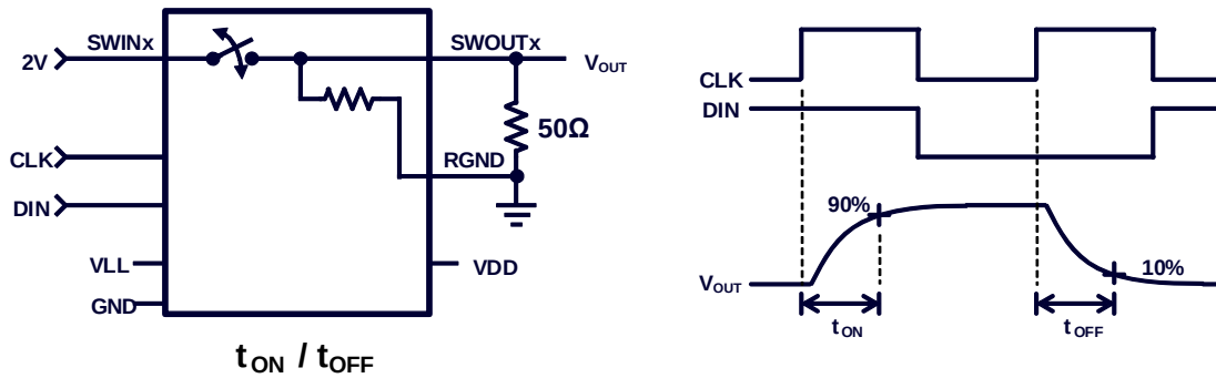
Figure 5: Test Circuit 4
