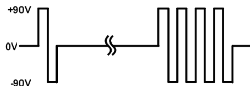
Figure 12: Typical High Voltage Burst
