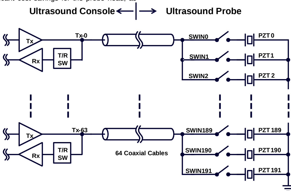
Figure 17: The MP4865A inside the Ultrasound Probe Head
