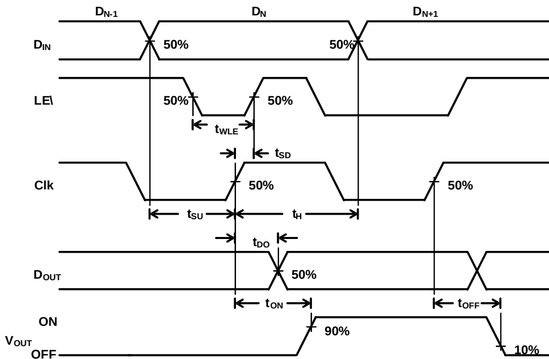
Figure 1: Timing Diagrams
