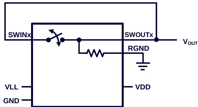
Figure 4: Test Circuit 3
