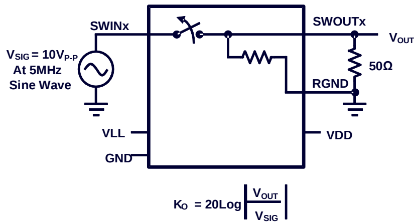
Figure 6: Test Circuit 5
