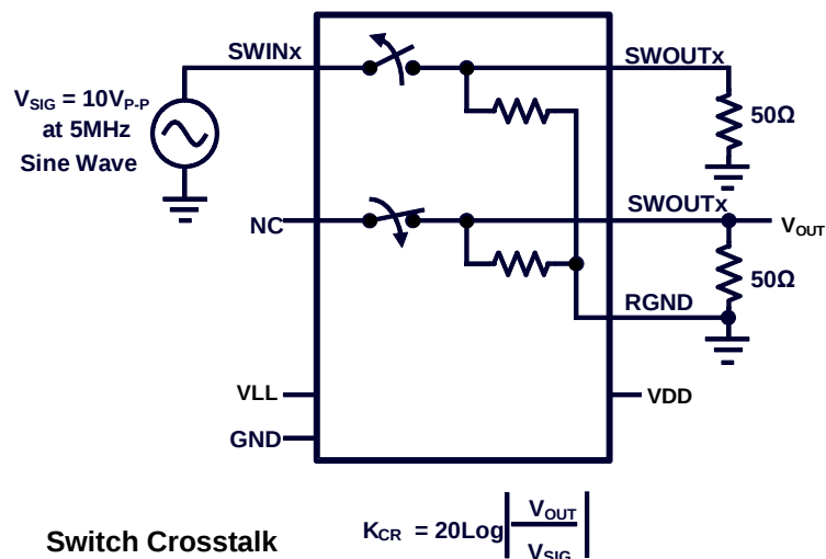
Figure 7: Test Circuit 6
