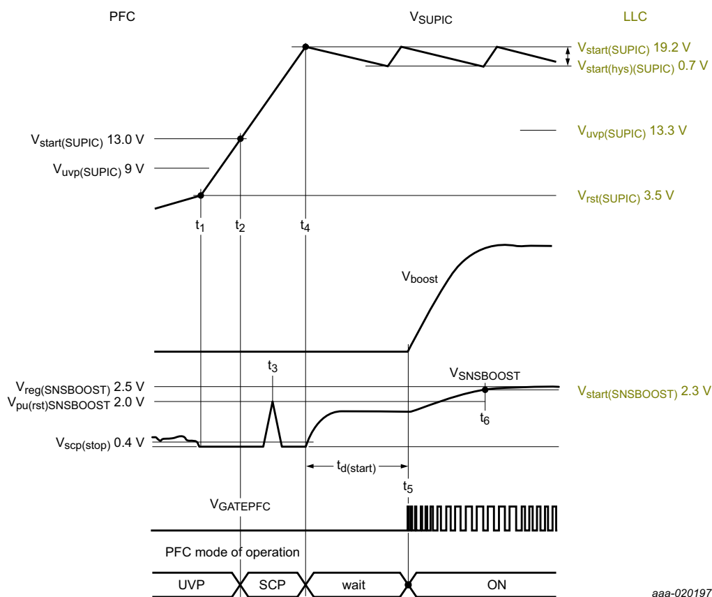
Fig 4. Start-up of the PFC and LLC
