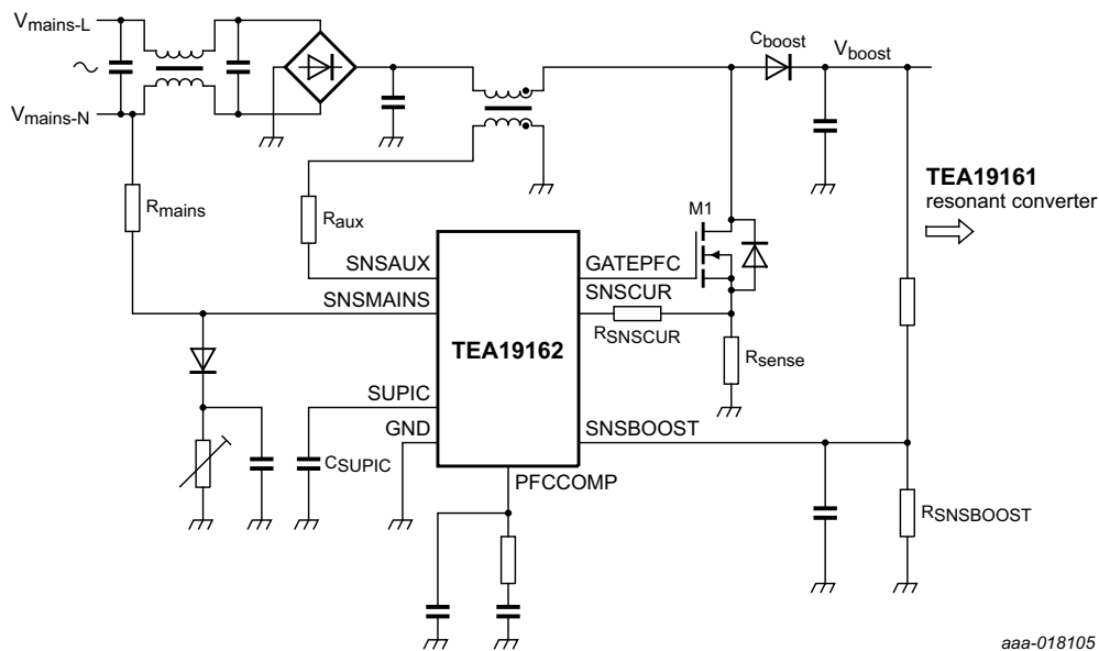
Fig 13. Application diagram
