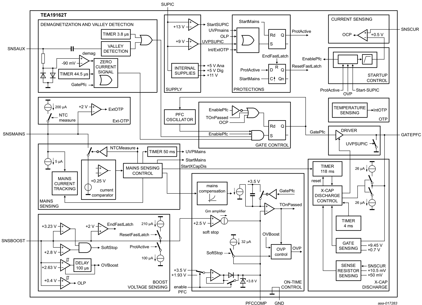
Fig 1. Block diagram
