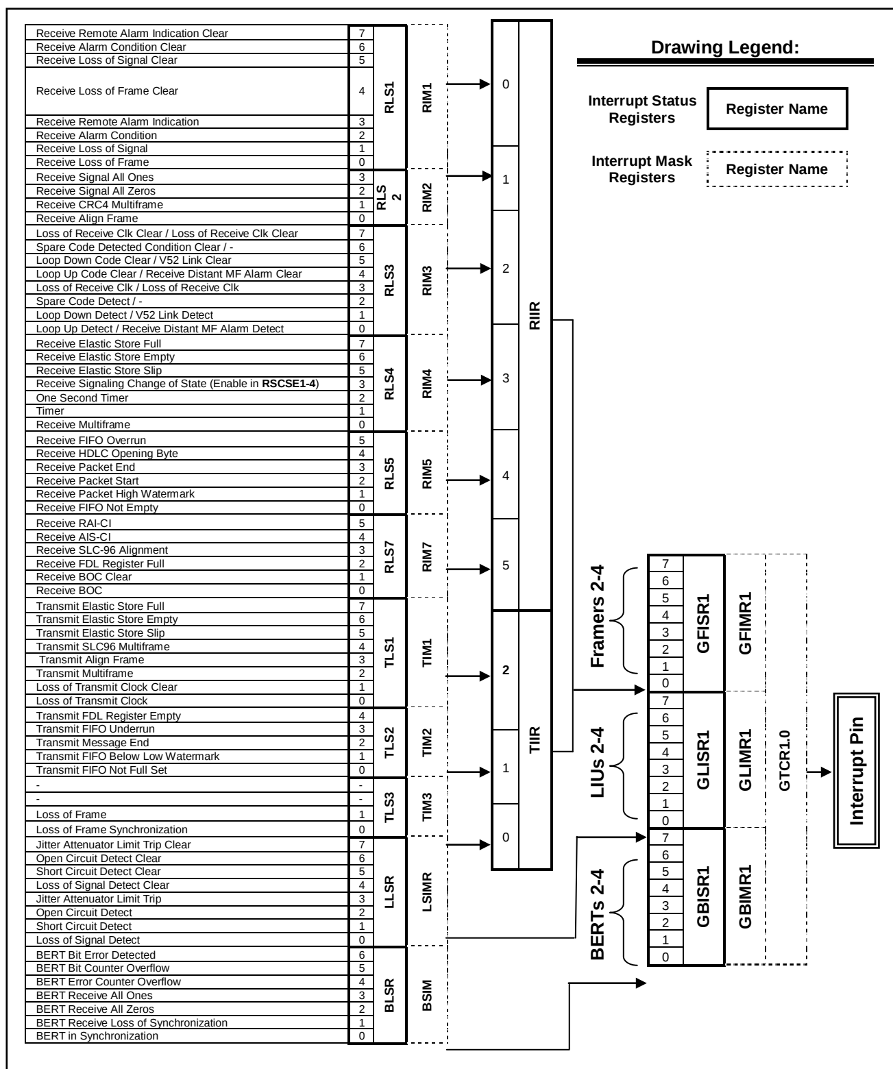
Figure 9-10. Device Interrupt Information Flow Diagram
