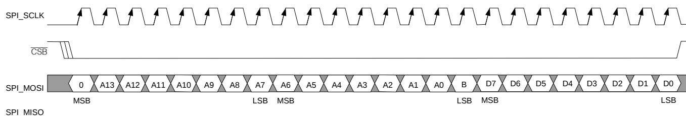
Figure 9-6. SPI Serial Port Access for Write Mode, SPI_CPOL = 1, SPI_CPHA = 0
