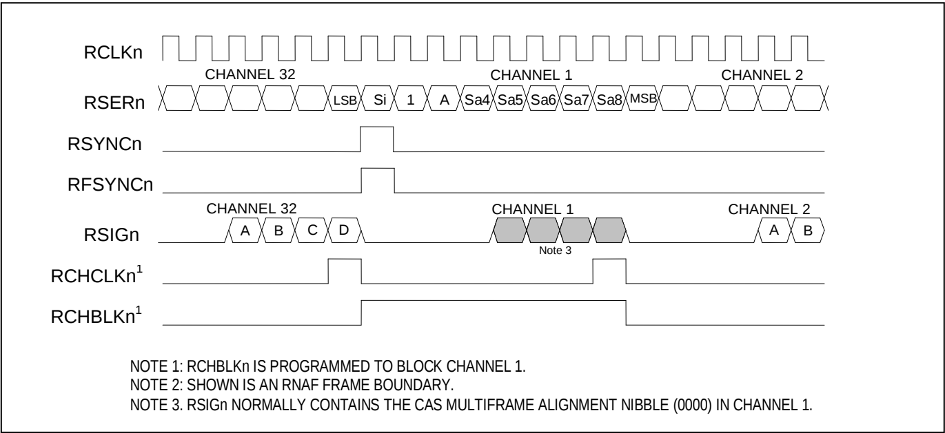
Figure 11-18. E1 Receive-Side Boundary Timing (Elastic Store Disabled)
