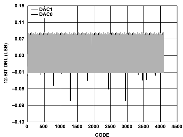
Figure 45. DNL, I_{OUTFS} = 20 mA, 12-Bit Resolution
