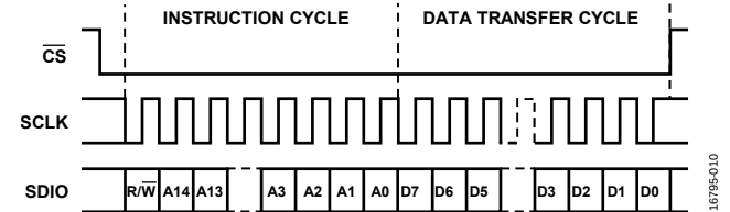
Figure 50. Serial Register Interface Timing, MSB First, Register 0x000, Bit 6 and Bit 1 = 0
