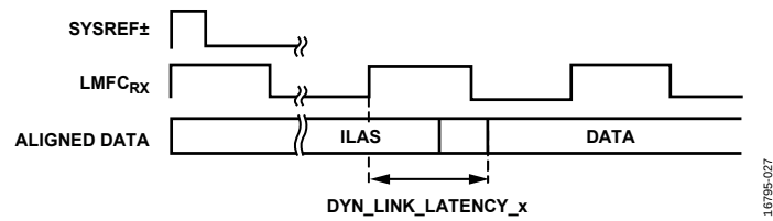
Figure 69. DYN_LINK_LATENCY_x Illustration
