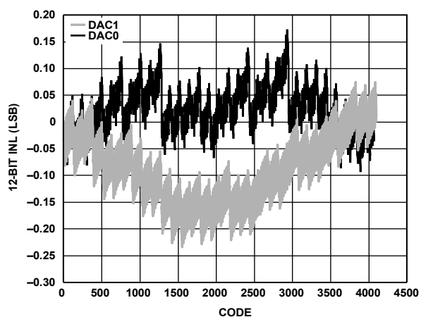
Figure 46. INL, I_{OUTFS} = 20 mA, 12-Bit Resolution
