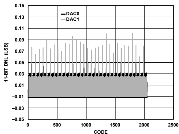
Figure 47. DNL, I_{OUTFS} = 20 mA, 11-Bit Resolution
