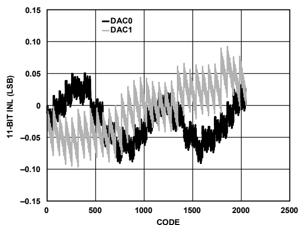
Figure 48. INL, I_{OUTFS} = 20 mA, 11-Bit Resolution
