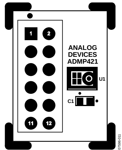
Figure 11. ADMP421 Evaluation Board Layout
