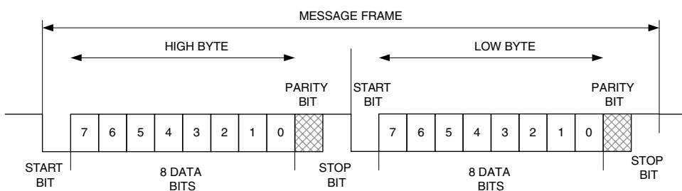
Figure 8. Command Bits
