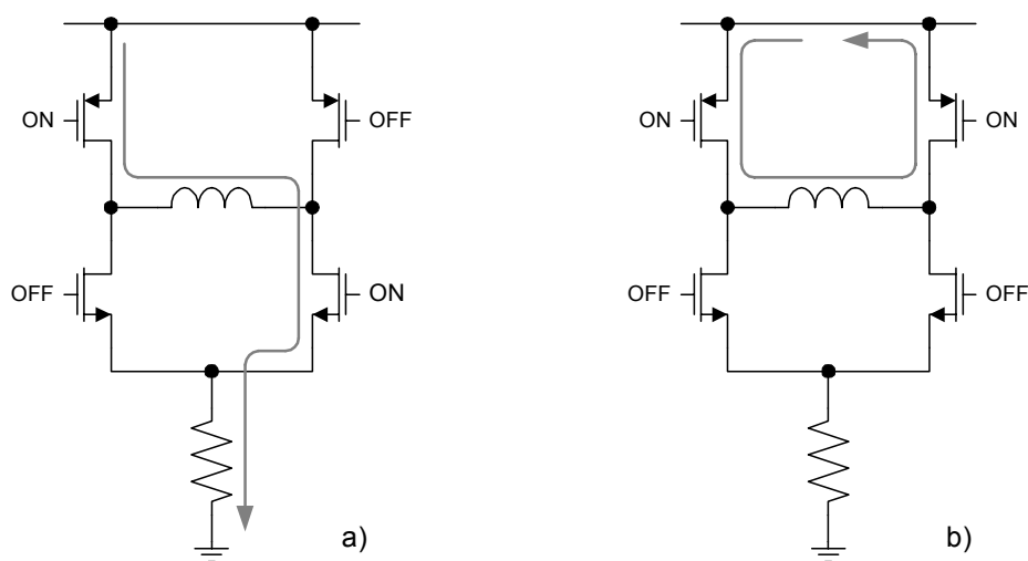
Figure 14. Current Flow in Halfbridge
