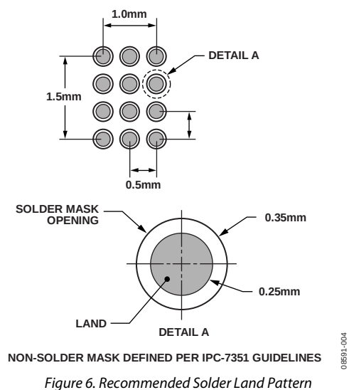
Figure 6. Recommended Solder Land Pattern
