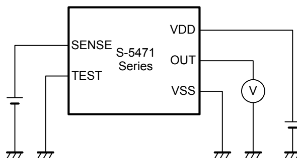
Figure 4 Test Circuit 2
