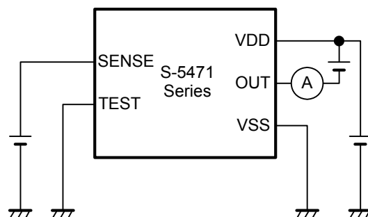
Figure 6 Test Circuit 4
