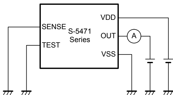
Figure 7 Test Circuit 5
