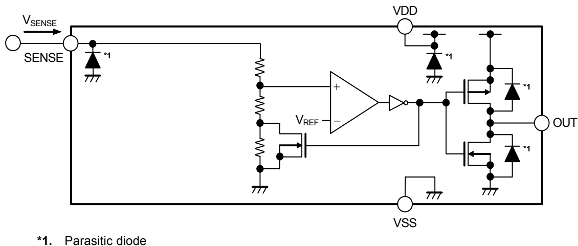
Figure 9 Explanatory Diagram for Operation at Voltage Detection
