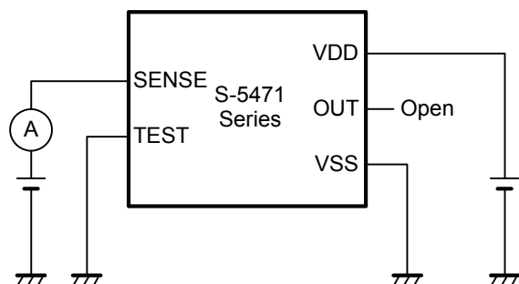
Figure 5 Test Circuit 3
