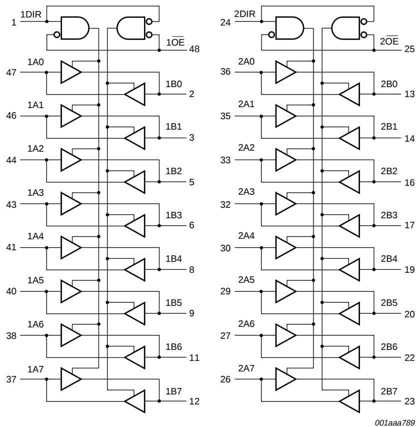
Fig 4. Logic diagram.
