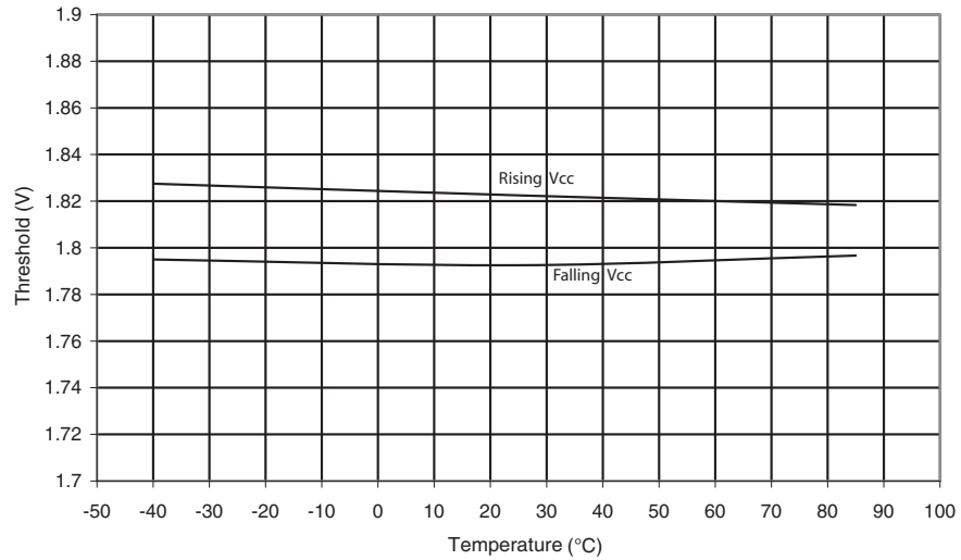
Figure 30-123. BOD Thresholds vs. Temperature (BODLEVEL is 1.8 V).
