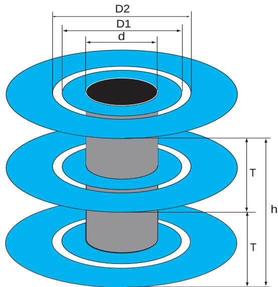
Figure 14: Via Construction
