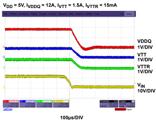
FIGURE 13. POWER-DOWN WAVEFORMS
