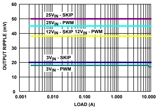
FIGURE 7. OUTPUT RIPPLE vs LOAD (1.8V) ( t_{ON} = GND )
