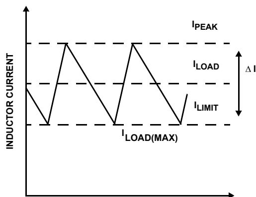
FIGURE 24. VALLEY CURRENT-LIMIT THRESHOLD
