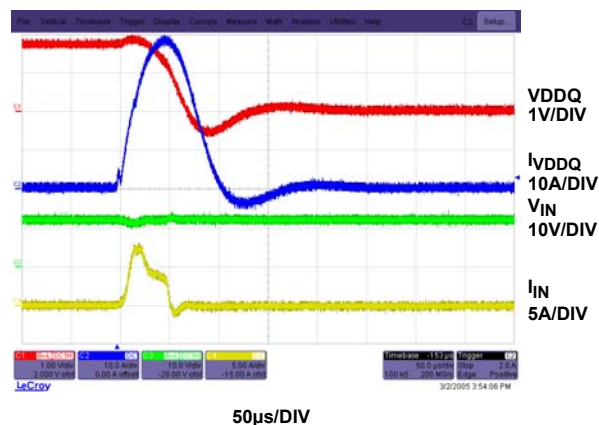
FIGURE 19. SHORT CIRCUIT AND RECOVERY OF VDDQ
