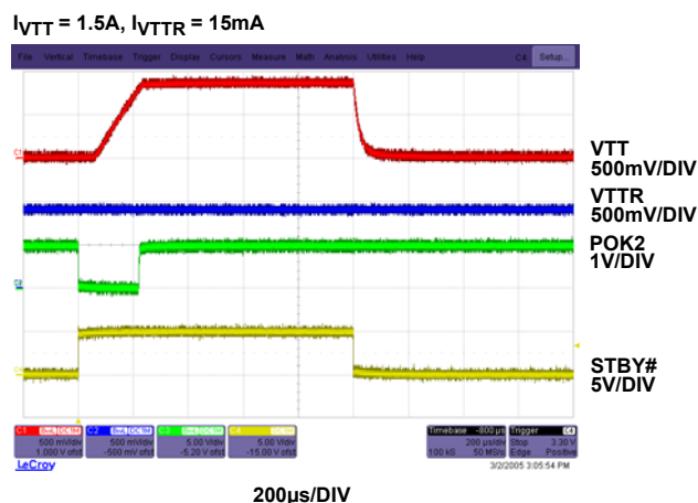
FIGURE 16. VTT, VTTR START-UP AND SHUTDOWN
