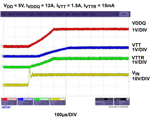
FIGURE 12. POWER-UP WAVEFORMS
