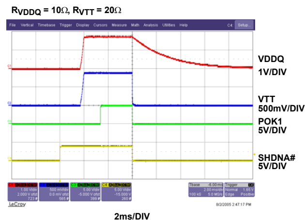
FIGURE 15. VDDQ START-UP AND SHUTDOWN INTO LIGHT LOAD, DISCHARGE ENABLED
