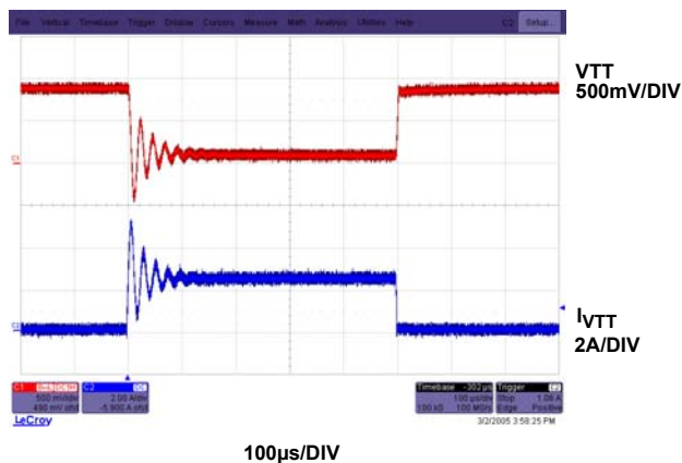
FIGURE 20. SHORT CIRCUIT AND RECOVERY OF VTT
