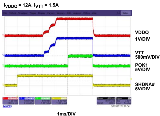
FIGURE 14. VDDQ START-UP AND SHUTDOWN INTO HEAVY LOAD, DISCHARGE DISABLED
