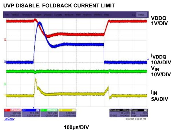
FIGURE 18. SHORT CIRCUIT AND RECOVERY OF VDDQ
