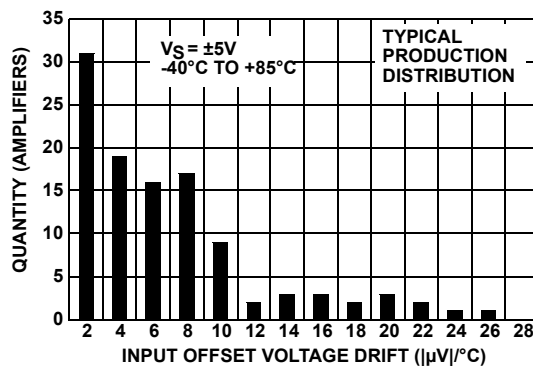
FIGURE 2. INPUT OFFSET VOLTAGE DRIFT (TSSOP, SOIC)
