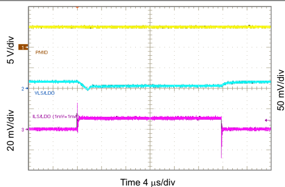
Figure 10-48. 1.2 V_{\text{LSLDO}} Load Transient, 0 to 10 mA
