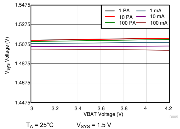
Figure 10-21. 1.5 V_{\text{SYS}} Line Regulation
