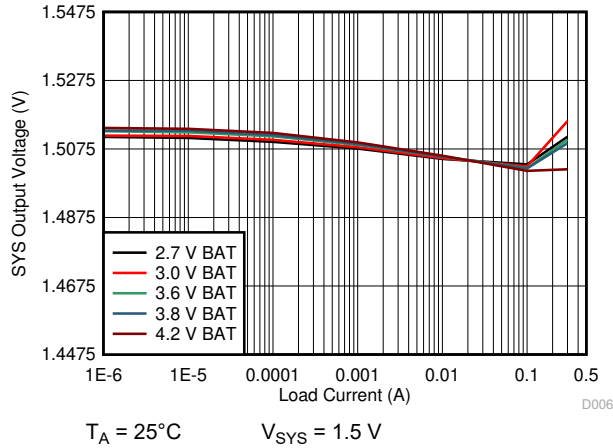
Figure 10-16. 1.5 V_{\text{SYS}} Load Regulation
