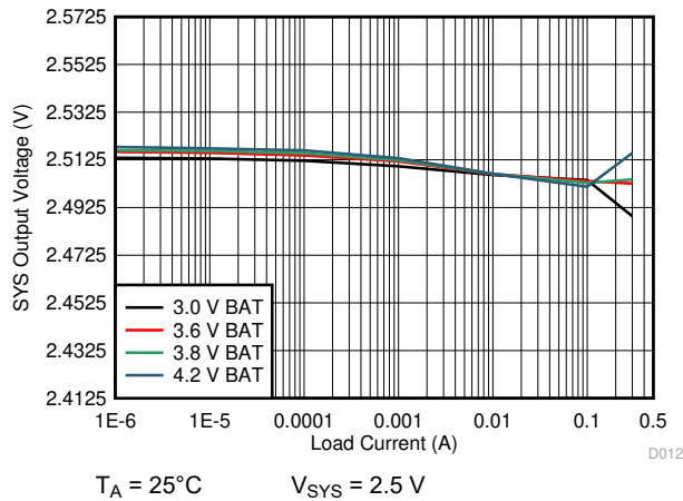
Figure 10-18. 2.5 V_{\text{SYS}} Load Regulation
