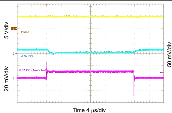
Figure 10-47. 0.8 V_{\text{LSLDO}} Load Transient, 0 to 10 mA
