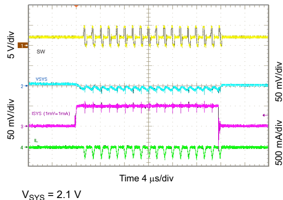
Figure 10-35. 2.1 V_{SYS} Load Transient, 0 to 50 mA
