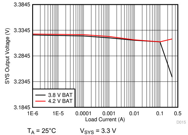
Figure 10-19. 3.3 V_{\text{SYS}} Load Regulation
