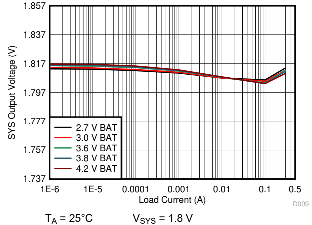
Figure 10-17. 1.8 V_{\text{SYS}} Load Regulation
