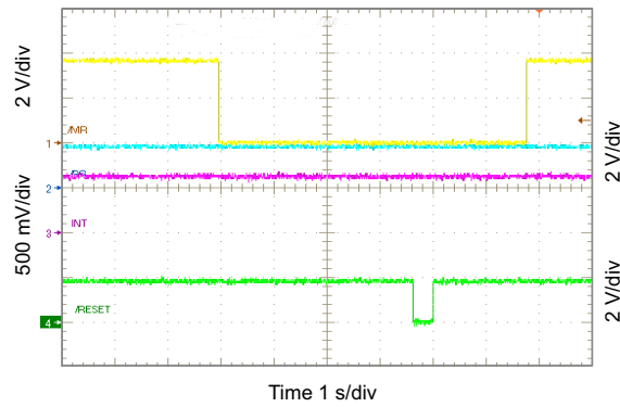
Figure 10-65. RESET Timing
