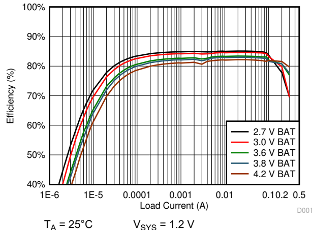
Figure 10-10. 1.2 V SYS System Efficiency
