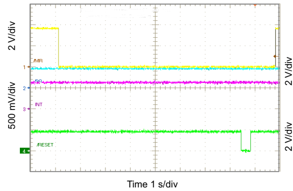
Figure 10-66. RESET Timing
