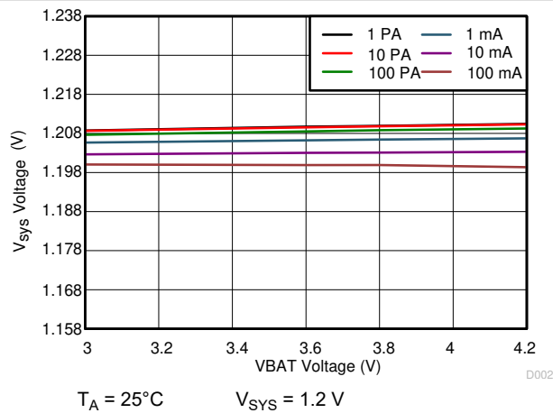
Figure 10-20. 1.2 V_{\text{SYS}} Line Regulation
