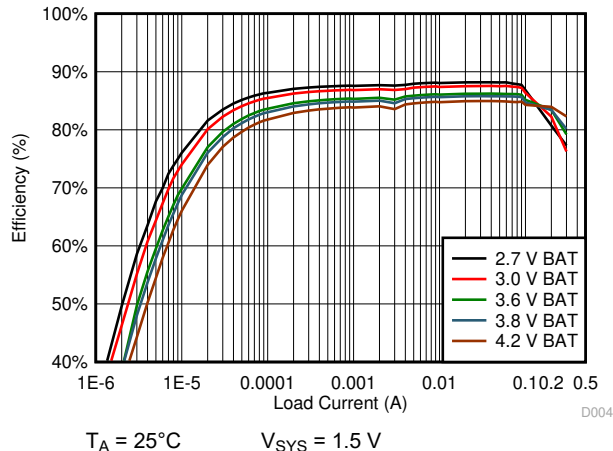
Figure 10-11. 1.5 V SYS System Efficiency
