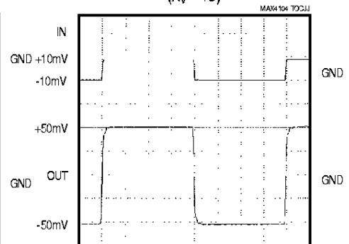
MAX4105 SMALL-SIGNAL PULSE RESPONSE ( A_V = +5 )
