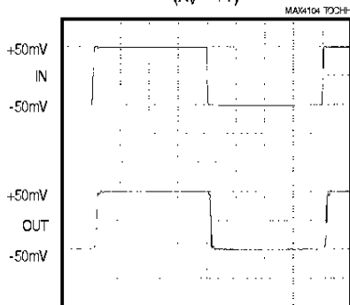
MAX4104 SMALL-SIGNAL PULSE RESPONSE ( A_V = +1 )
