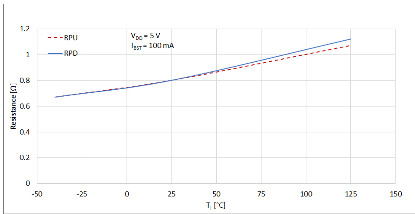
Figure 20 BST pull-up and pull-down resistance versus temperature
