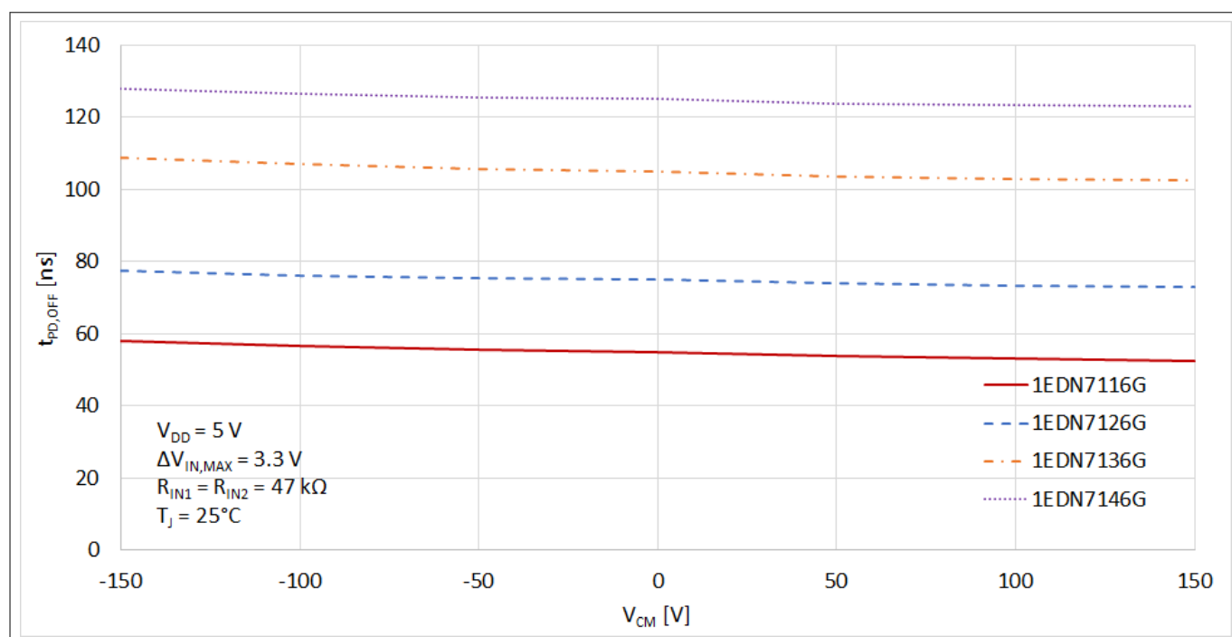
Figure 16 Turn-off propagation delay versus common mode voltage
