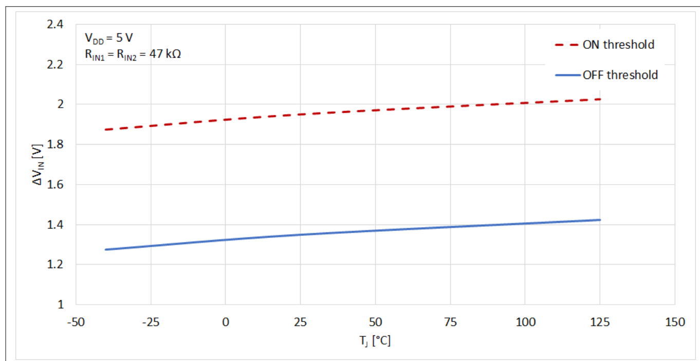
Figure 7 Differential input voltage threshold versus temperature
