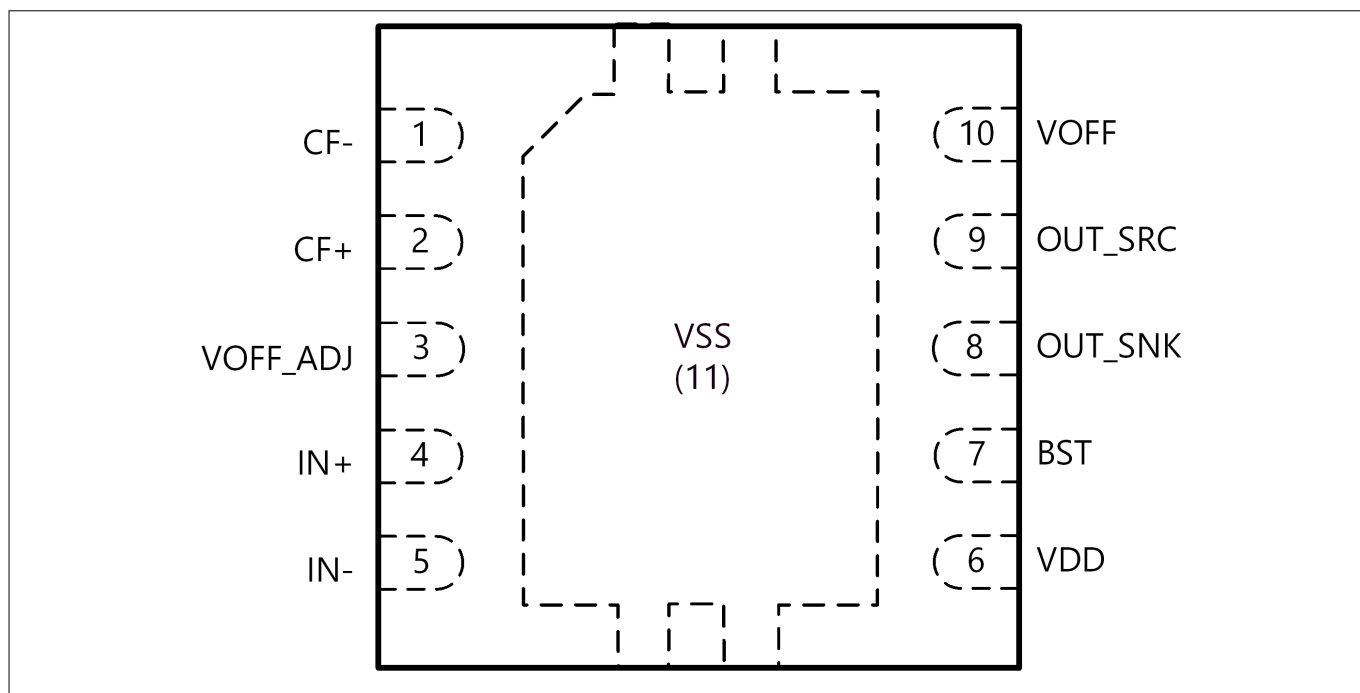
Figure 1 Pin configuration 1EDN71X6G in PG-VSON-10 package, top view
