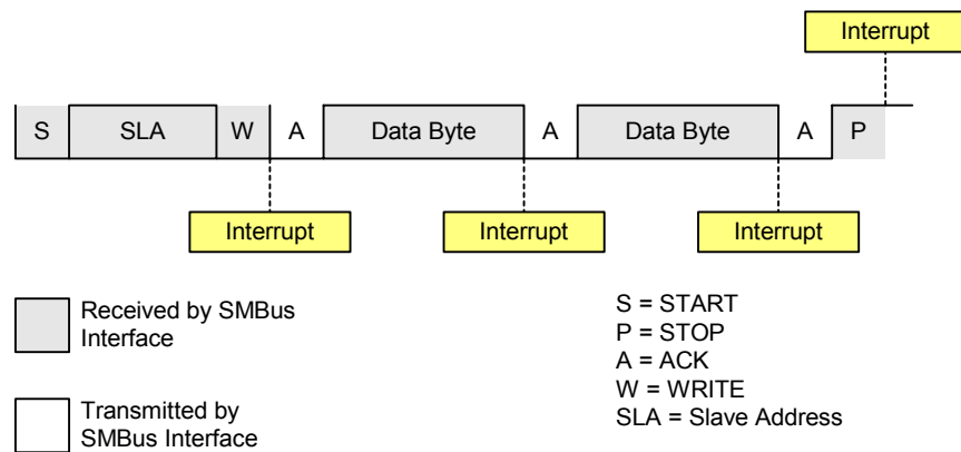
Figure 16.10. Typical Slave Receiver Sequence
