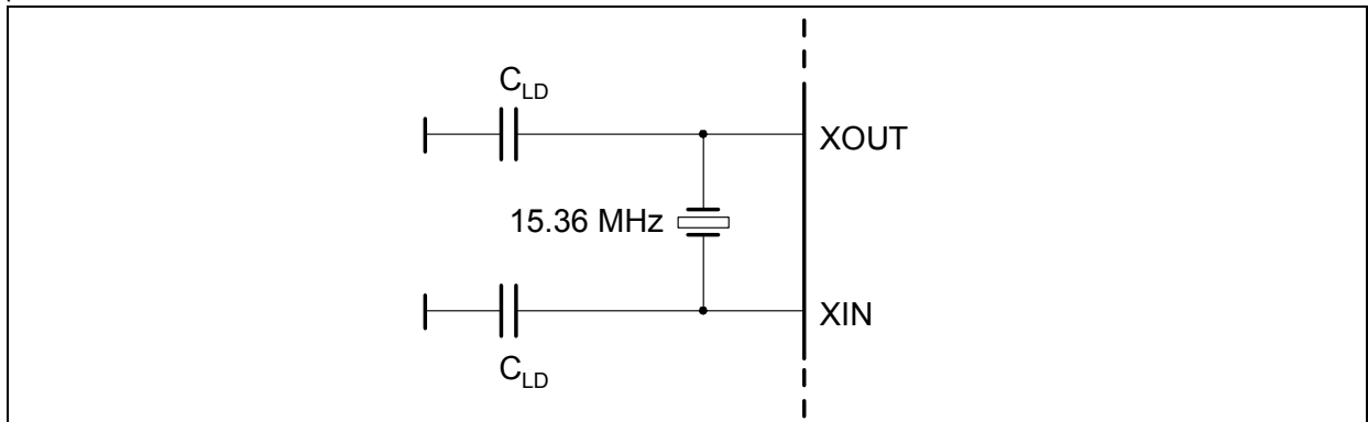
Figure 22 Crystal Oscillator
