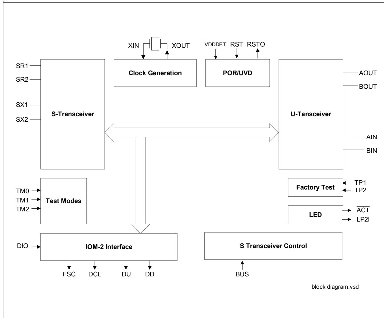
Figure 2 Block Diagram
