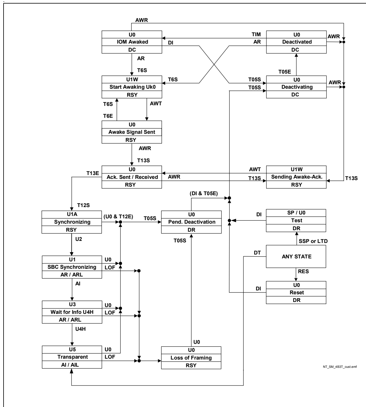
Figure 8 NT State Machine (IEC-T/NTC-T Compatible)
