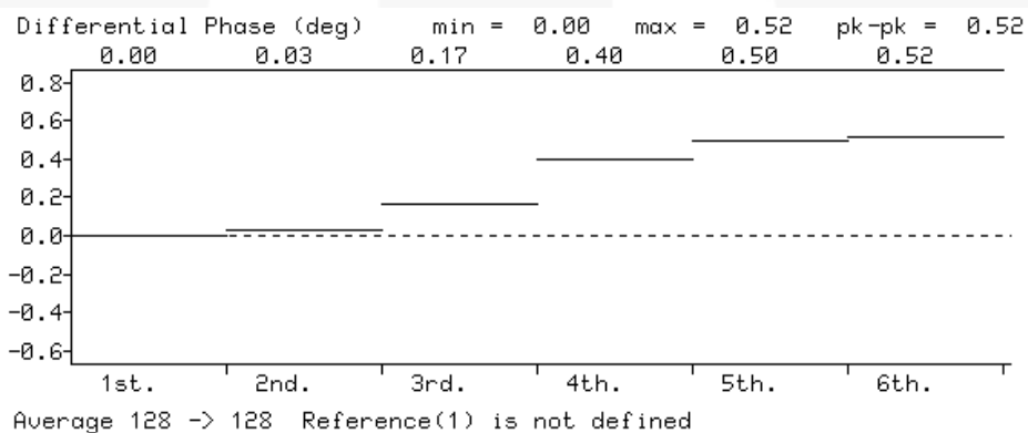
Figure 10. Differential Phase
