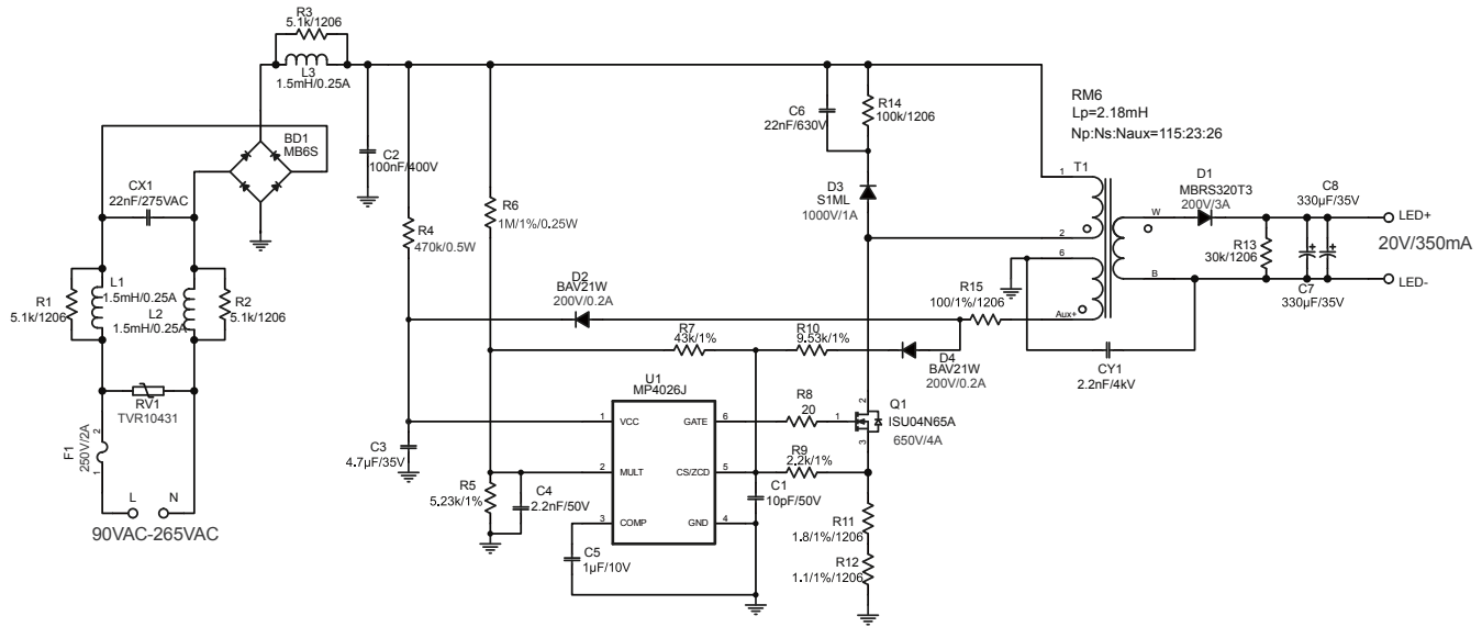
Figure 14: A19 Bulb Driver, 90-265VAC Input, Isolated Flyback Converter, V_O = 20V , I_O = 350mA EV Model: EV4026-J-00A
