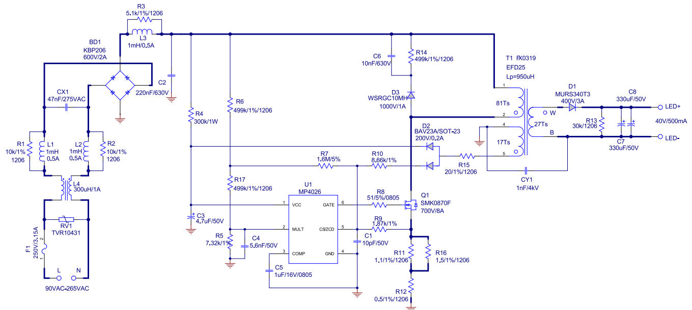
Figure 15: PAR38 Driver, 90-265VAC Input, Isolated Flyback Converter, V_O = 40V , I_O = 500mA EV Model: EV4026-J-00B
