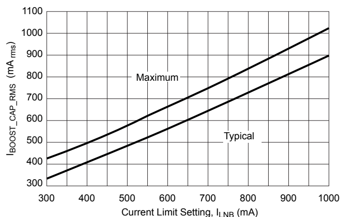
Figure 10. Boost capacitor rms current versus I_{\text{LNB}}
