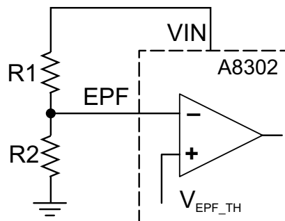
Figure 7. Example circuit for Early Power Failure feature
