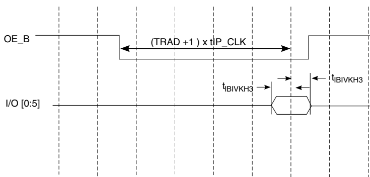
Figure 38. IFC-NAND interface input AC timings
