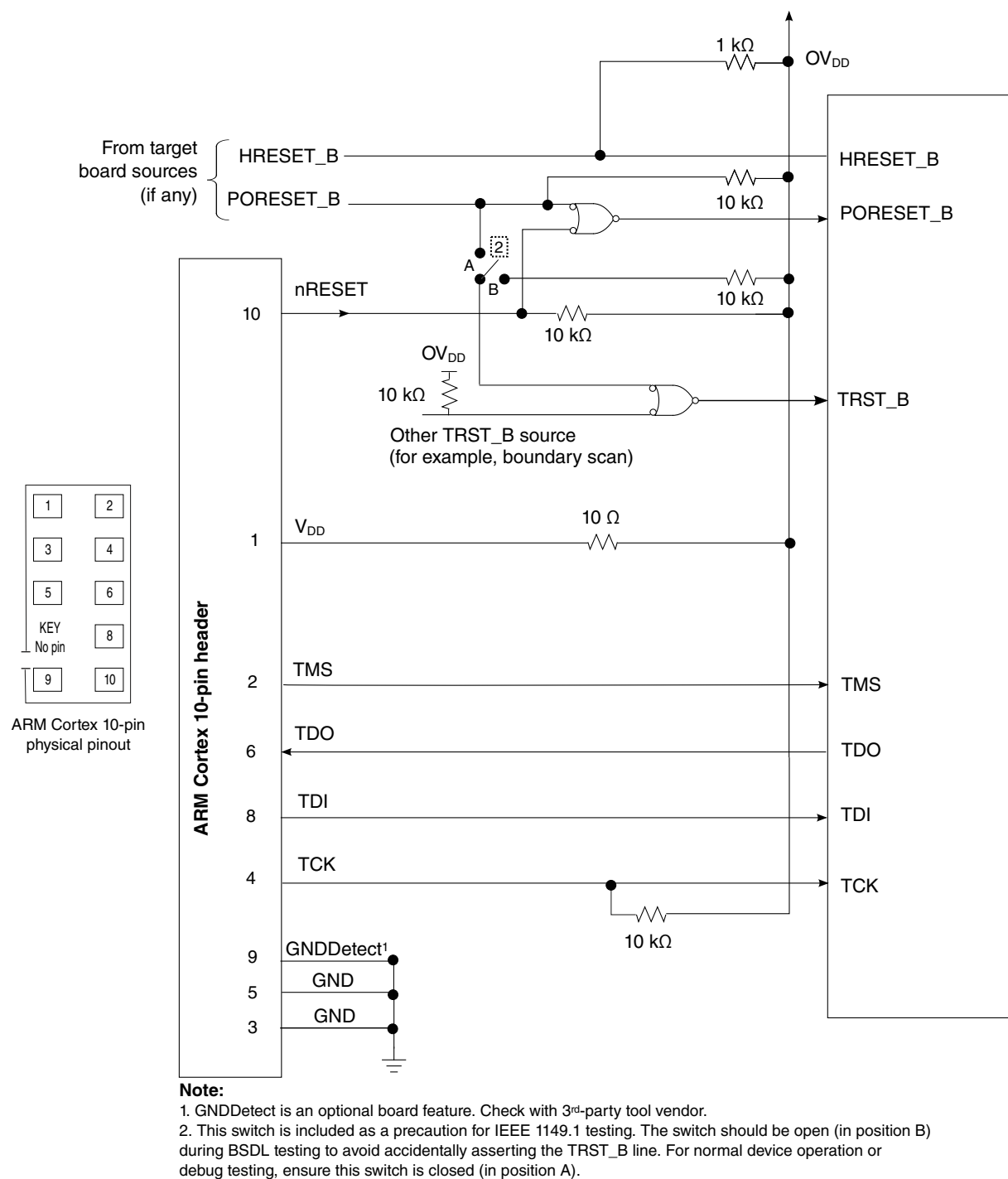
Figure 88. JTAG interface connection
