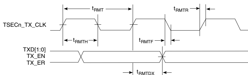
Figure 22. RMII transmit AC timing diagram
