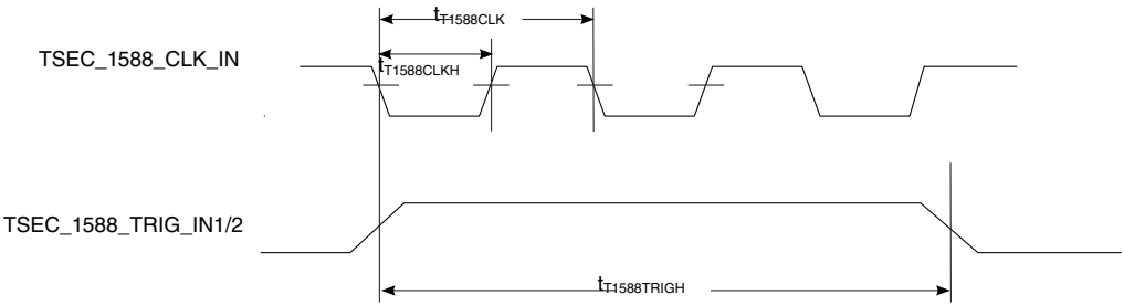
Figure 26. IEEE 1588 input AC timing
