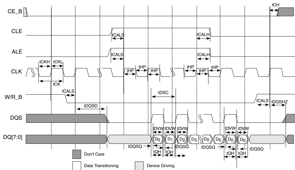
Figure 45. Read cycle
