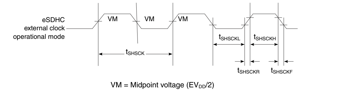
Figure 56. eSDHC clock input timing diagram
