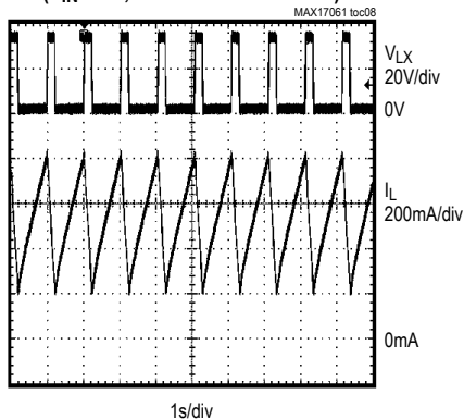
SWITCHING WAVEFORMS ( V_{IN} = 7V , BRIGHTNESS = 100%)
