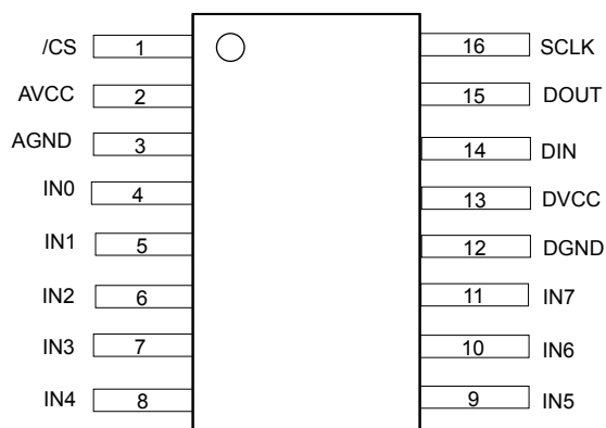
Figure 1. Pin description (top view)
