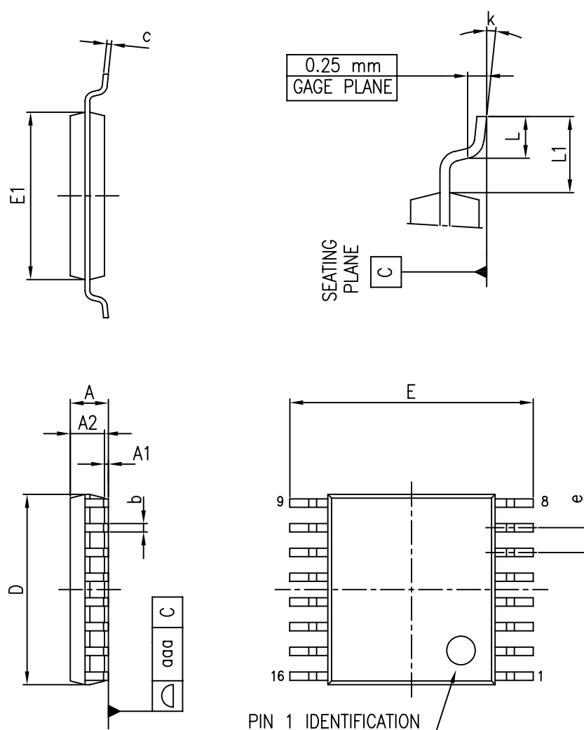
Figure 4. TSSOP-16 package outline
