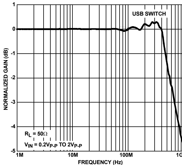
FIGURE 33. FREQUENCY RESPONSE
