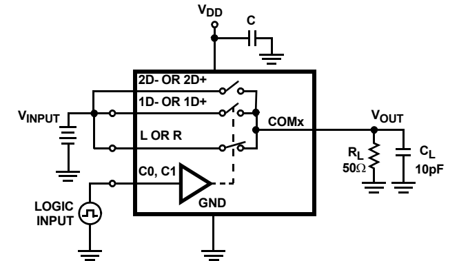
FIGURE 1. SWITCHING TIMES
