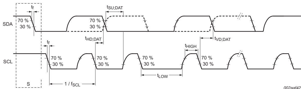
Fig 27. I 2 C-bus pins clock timing
