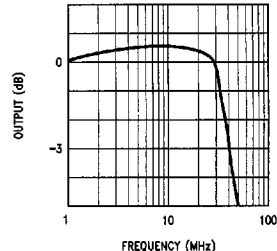
LM2416 Frequency Response
