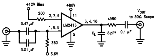
FIGURE 1. Test Circuit (One Section)
