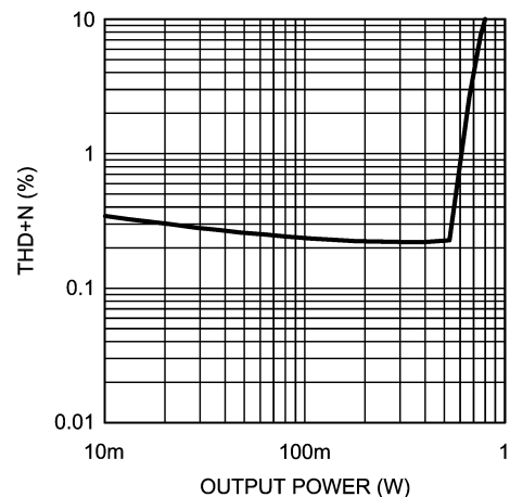
THD+N vs Output Power V_{DD} = 3V , R_L = 4\Omega , and f = 1kHz
