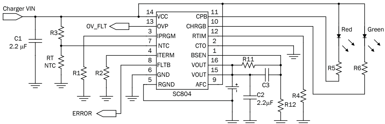
Figure 3a - Application Circuit for Adjust Mode
