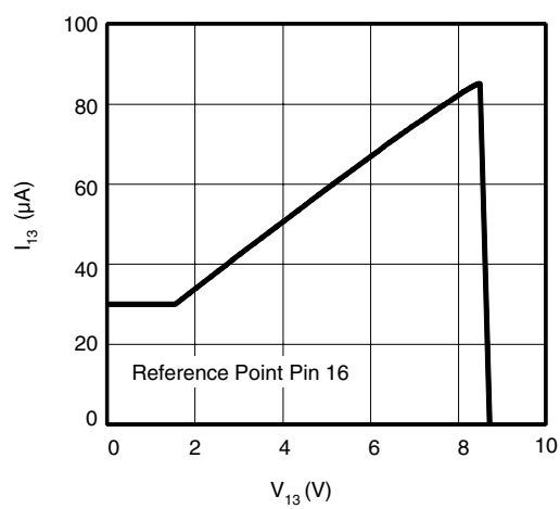
Figure 10. Soft-start Charge Current (f/V Converter Non-active)
