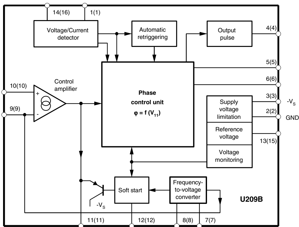
Figure 1. Block Diagram
