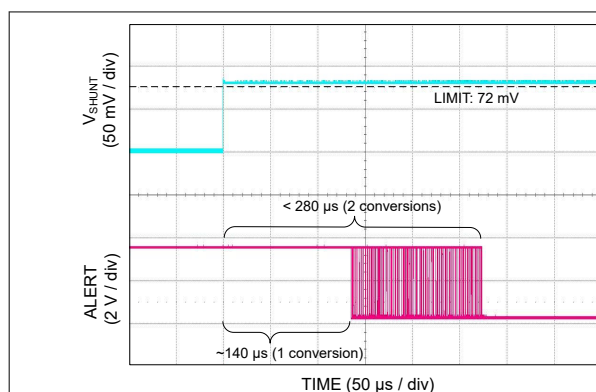
Figure 8-3. Alert Response ( t_{CT} = 140 \text{ } \mu\text{s} )
