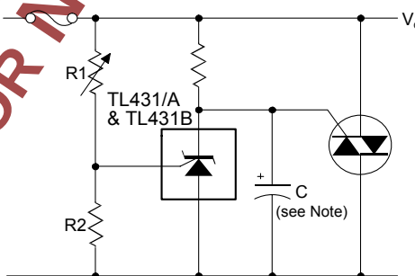
Figure 19 – Crowbar Circuit
