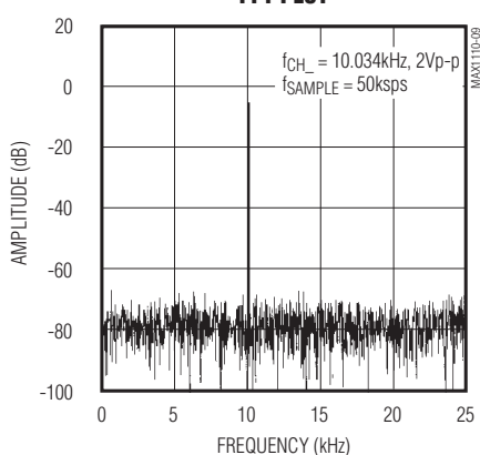
FFT PLOT
