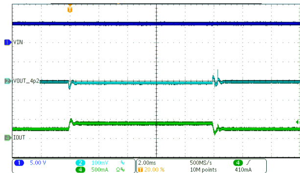
Figure 8-8. OUT Transient Response
