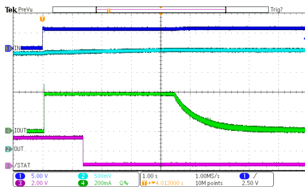
Figure 8-10. ISET Short-Circuit Response
