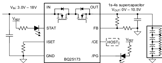
Simplified Schematic
