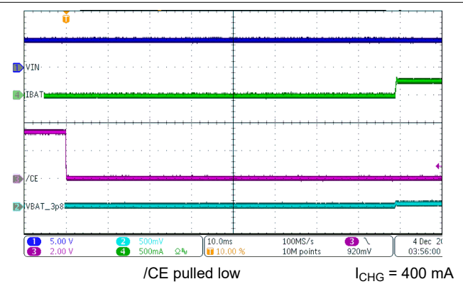
Figure 8-5. Charge Enable
